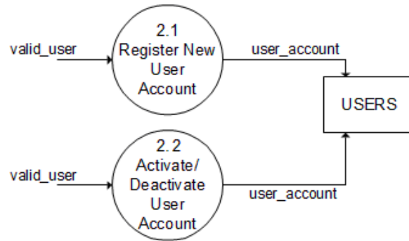
Figure 6: Sub explosion of Update User Accounts, Ortho-WISE
