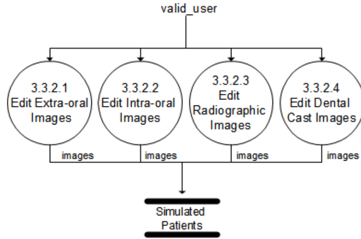
Figure 12: Sub explosion of Edit Images, Ortho-WISE
