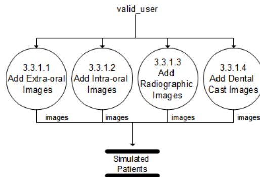
Figure 11: Sub explosion of Add Images, Ortho-WISE
