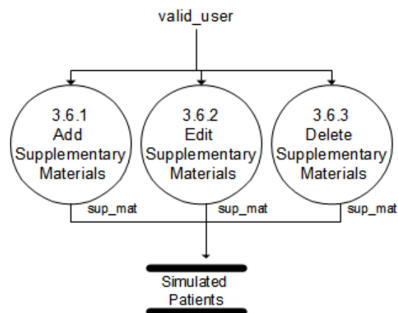
Figure 16: Sub explosion of Update Supplementary Materials, Ortho-WISE
