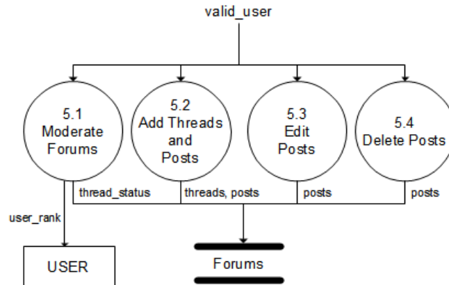
Figure 22: Sub explosion of Participate in Forums, Ortho-WISE
