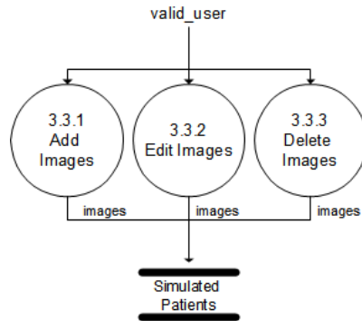
Figure 10: Sub explosion of Update Patient Images, Ortho-WISE
