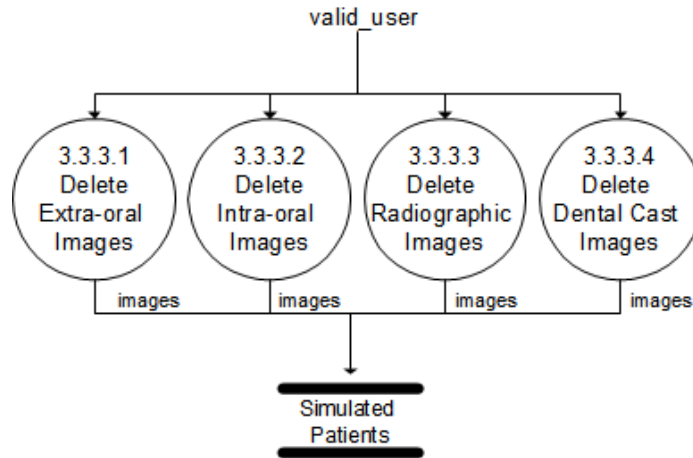
Figure 13: Sub explosion of Delete Images, Ortho-WISE
