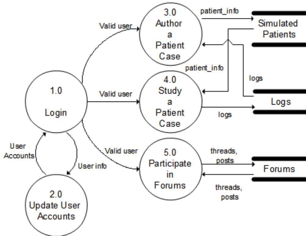
Figure 4: Top Level Data Flow Diagram, Ortho-WISE
