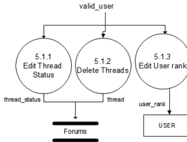
Figure 23: Sub explosion of Moderate Forums, Ortho-WISE
