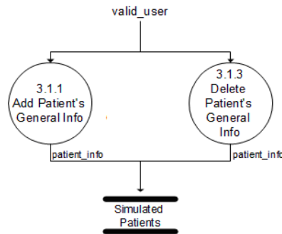
Figure 8: Sub explosion of Update Patient General Info, Ortho-WISE
