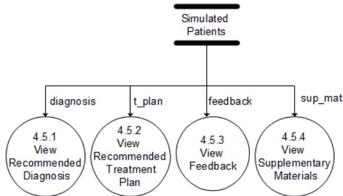
Figure 21: Sub explosion of View Activity Results, Ortho-WISE
