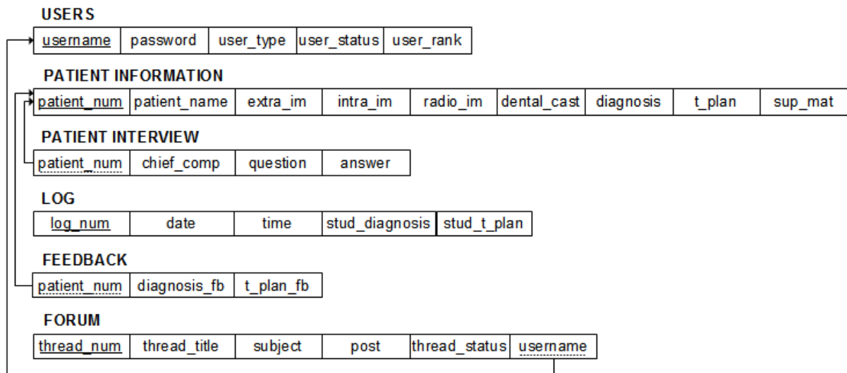
Figure 24: Relational Model, Ortho-WISE
