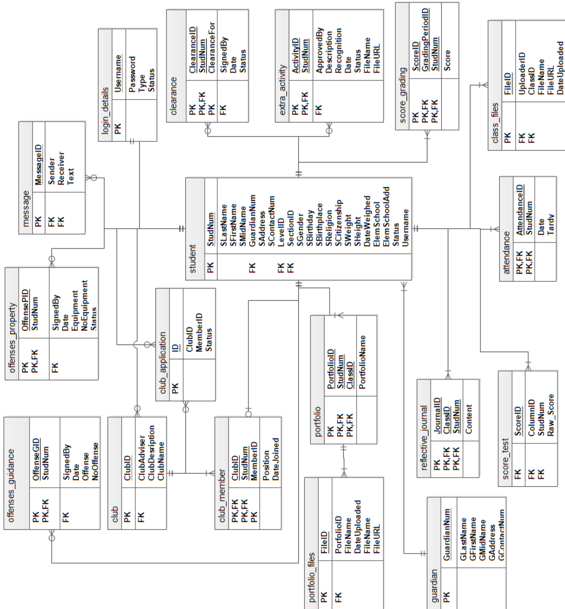
Figure 2: Entity Relationship Diagram Focused on Student, ValSci Student/Faculty Portal
