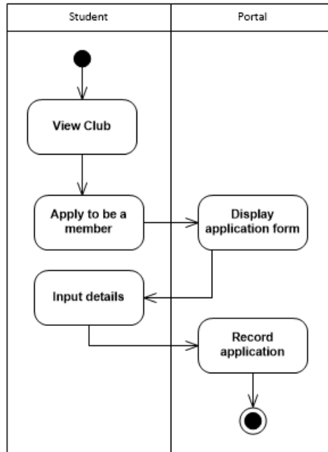
Figure 28: Applying for membership Manage Club Use Case , ValSci Student/Faculty Portal
