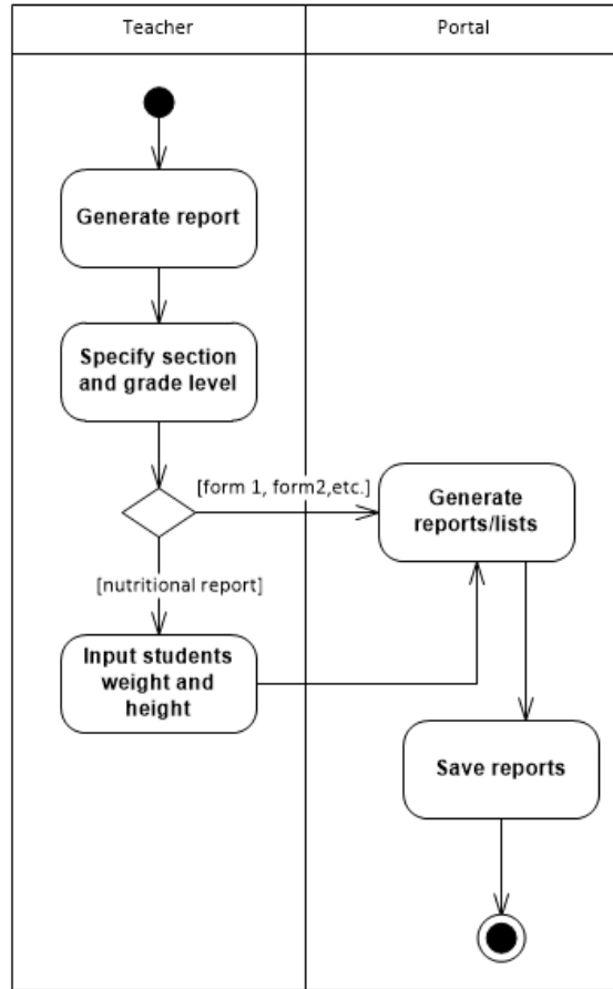
Figure 23: Generating reports in Manage Reports Use Case , ValSci Student/Faculty Portal
