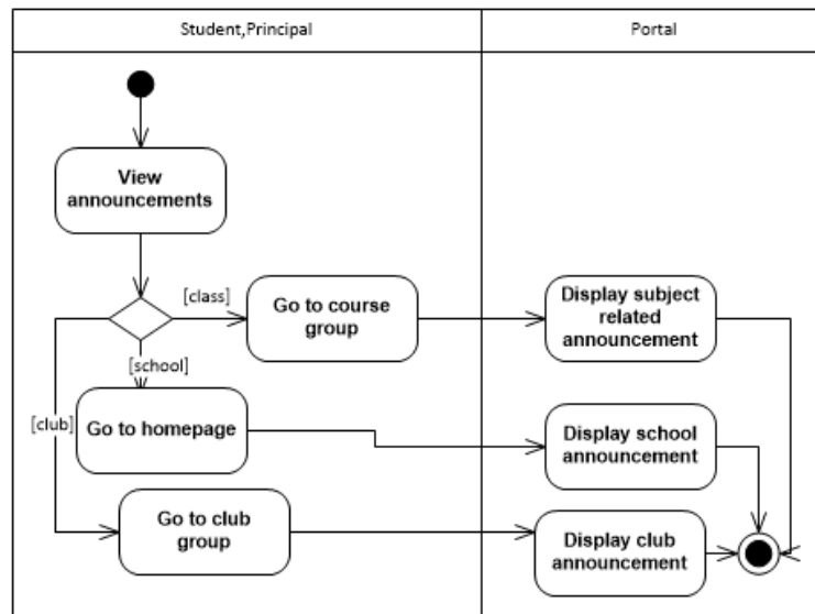
Figure 7: Viewing Announcements in Manage Messages Use Case , ValSci Student/Faculty Portal
