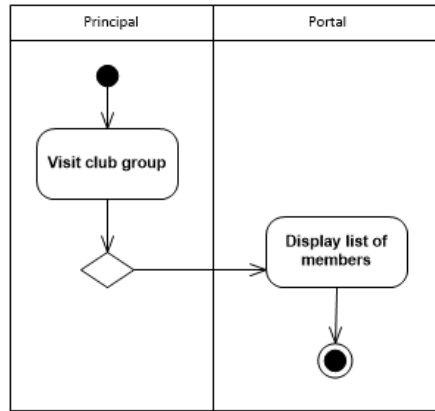
Figure 27: Viewing members of a club Manage Club Use Case , ValSci Student/Faculty Portal
