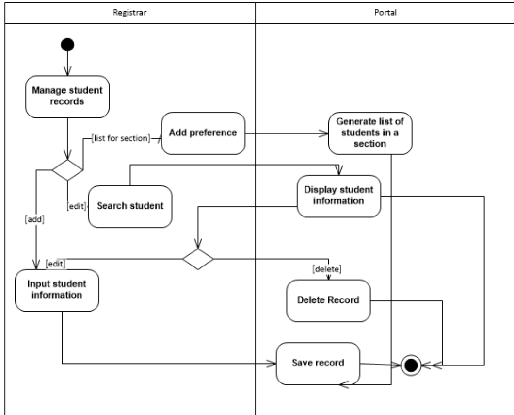
Figure 17: Sectioning, and creating, viewing, updating and deleting student record in Manage Student Records Use Case , ValSci Student/Faculty Portal
