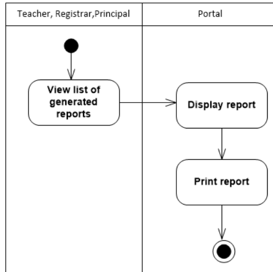
Figure 24: Viewing generated reports in Manage Reports Use Case , ValSci Student/Faculty Portal
