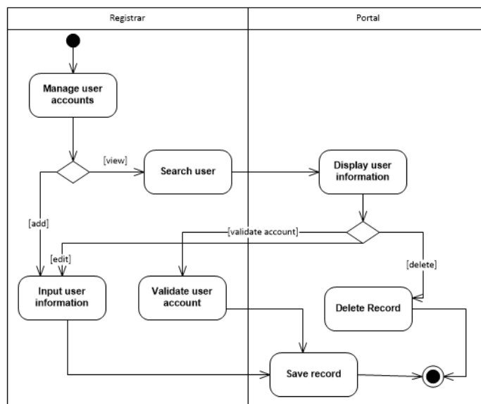
Figure 15: Creating, validating and deleting a user account in Manage Account Use Case , ValSci Student/Faculty Portal
