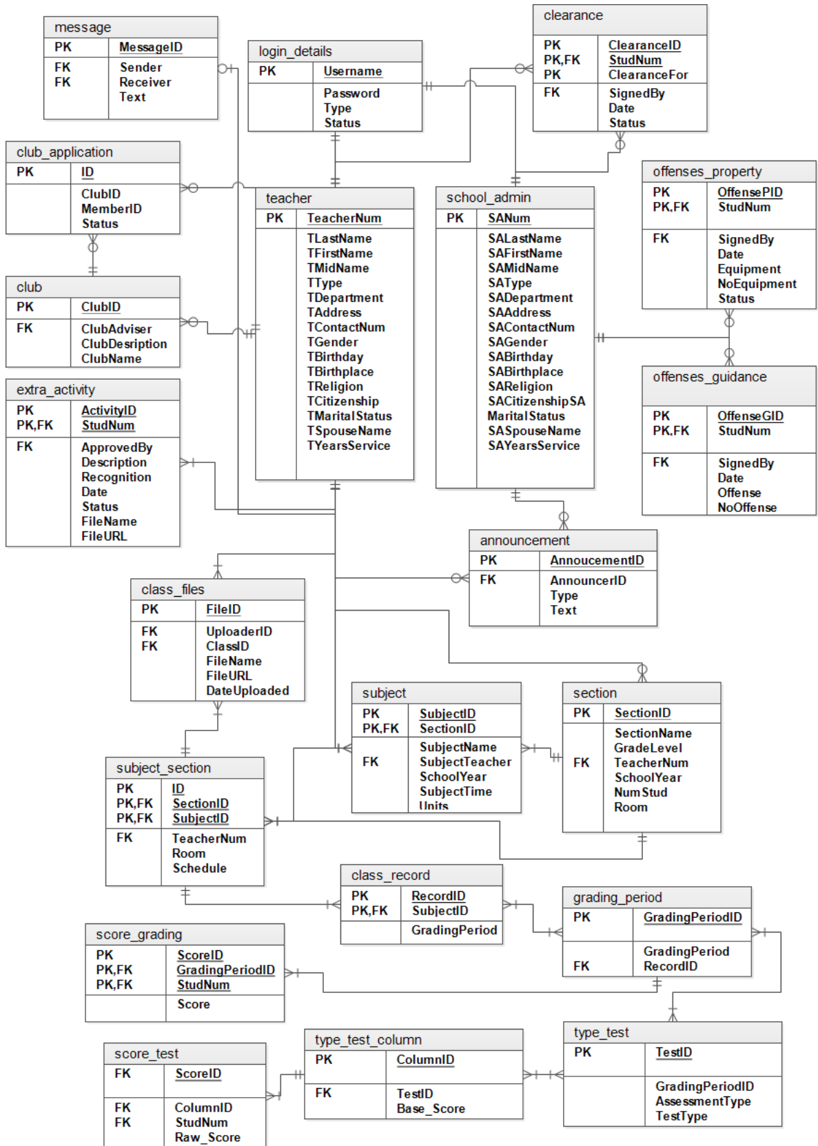
Figure 3: Entity Relationship Diagram Focused on School Administrators, ValSci Student/Faculty Portal
