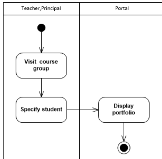
Figure 10: Viewing of portfolio in Manage Files Use Case , ValSci Student/Faculty Portal
