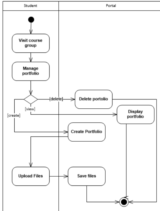
Figure 9: Creating and uploading files in portfolio in Manage Files Use Case , ValSci Student/Faculty Portal
