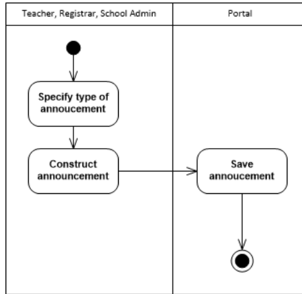
Figure 6: Adding announcements in Manage Messages Use Case , ValSci Student/Faculty Portal
