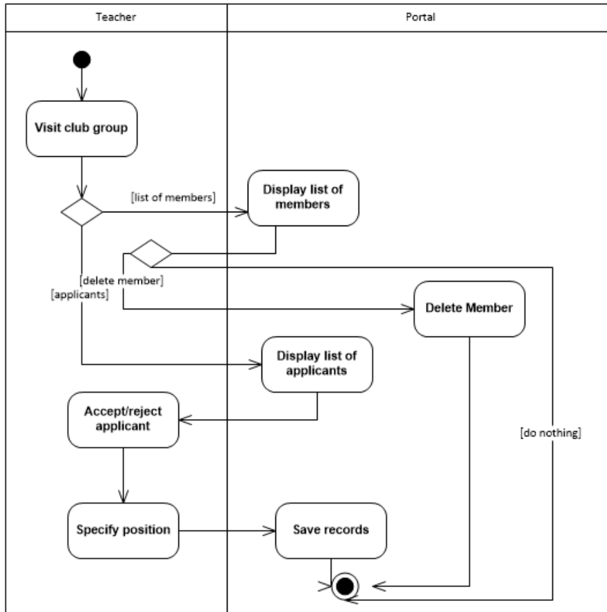
Figure 25: Viewing, deleting and accepting members in Manage Club Use Case , ValSci Student/Faculty Portal
