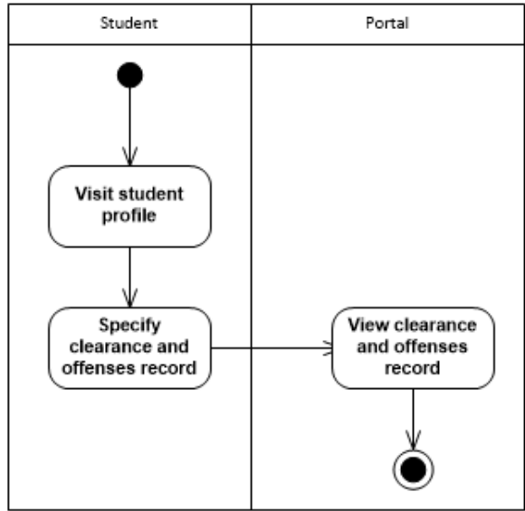
Figure 22: Viewing of student’s clearance and offenses record in Manage Student Records Use Case , ValSci Student/Faculty Portal
