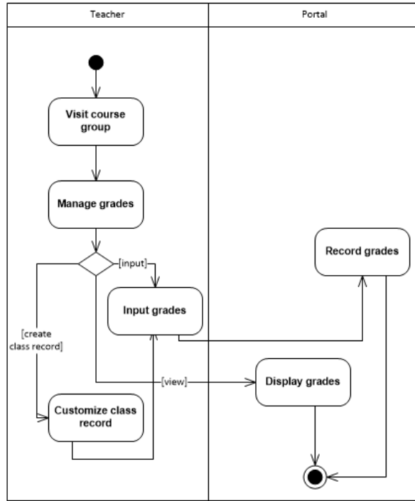
Figure 20: Creating class record and recording of grades in Manage Student Records Use Case , ValSci Student/Faculty Portal
