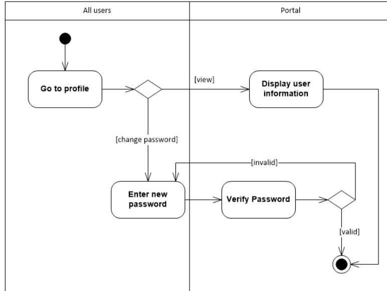
Figure 14: Changing password in Manage Account Use Case , ValSci Student/Faculty Portal
