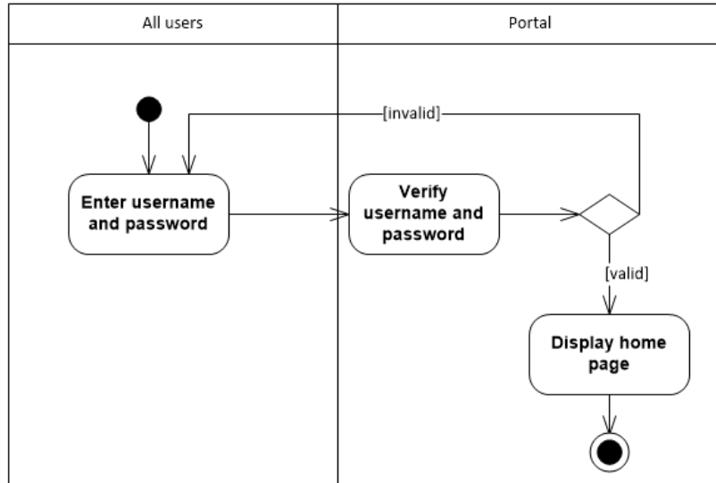
Figure 13: Logging in in Log-In Files Use Case , ValSci Student/Faculty Portal
