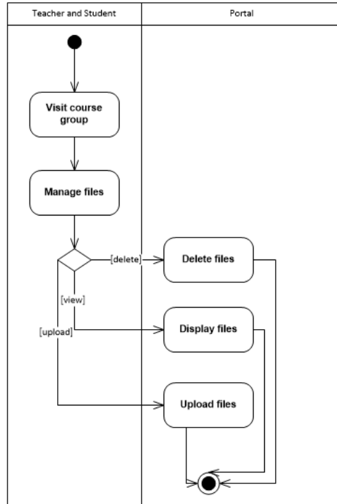
Figure 11: Viewing, uploading and deleting files in Manage Files Use Case , ValSci Student/ Faculty Portal
