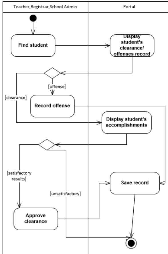
Figure 19: Recording of offenses and approving of clearance in Manage Student Records Use Case , ValSci Student/Faculty Portal
