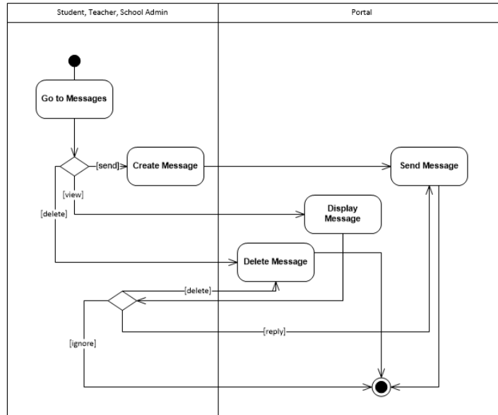
Figure 8: Viewing, creating and deleting messages in Manage Messages Use Case , ValSci Student/Faculty Portal
