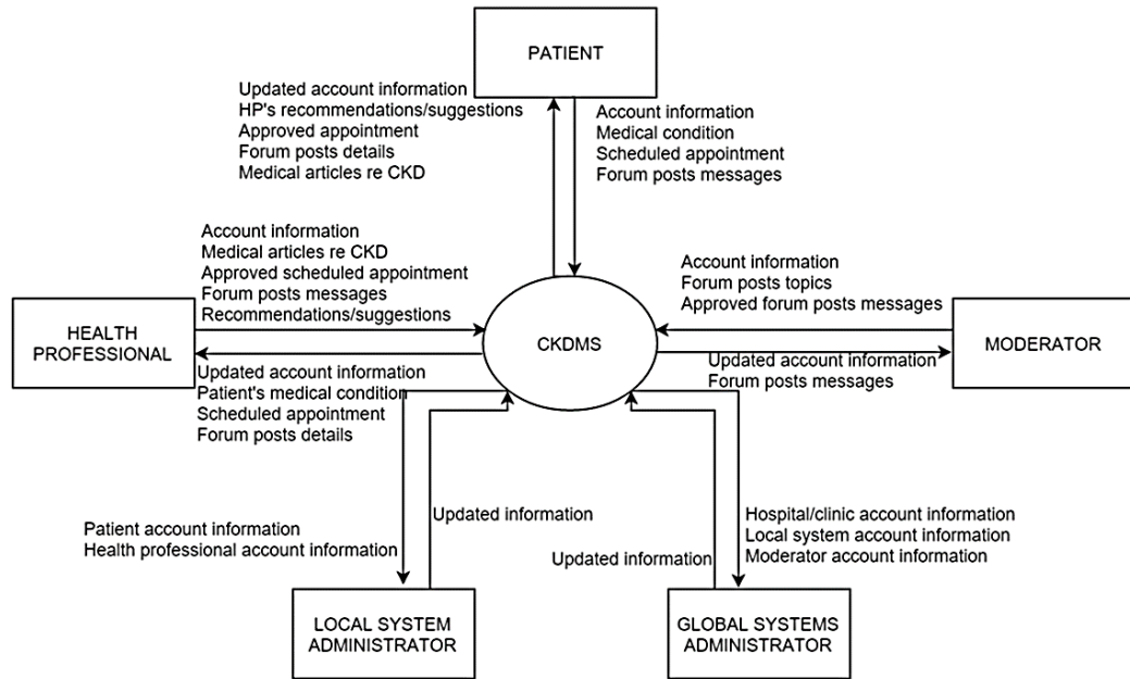
Figure 1: Context Diagram of CKDMS
