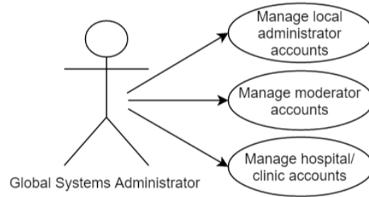
Figure 2: Use Case Diagram of CKDMS
