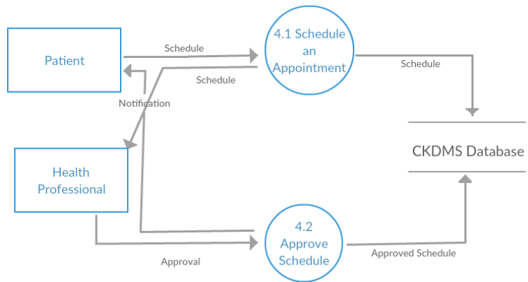
Figure 6: Sub-explosion for Manage Schedule Function of CKDMS
