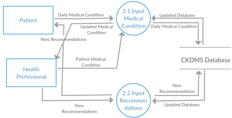
Figure 5: Sub-explosion for Update Medical Condition Function of CKDMS
