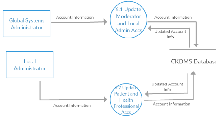
Figure 8: Sub-explosion for Manage Accounts Function of CKDMS
