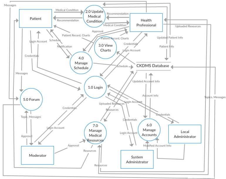
Figure 3: Data Flow Diagram of CKDMS
