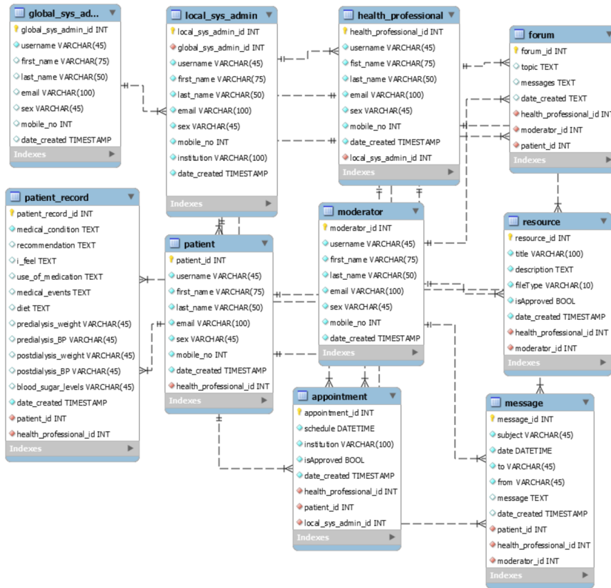
Figure 10: Entity Relationship Diagram of CKDMS
