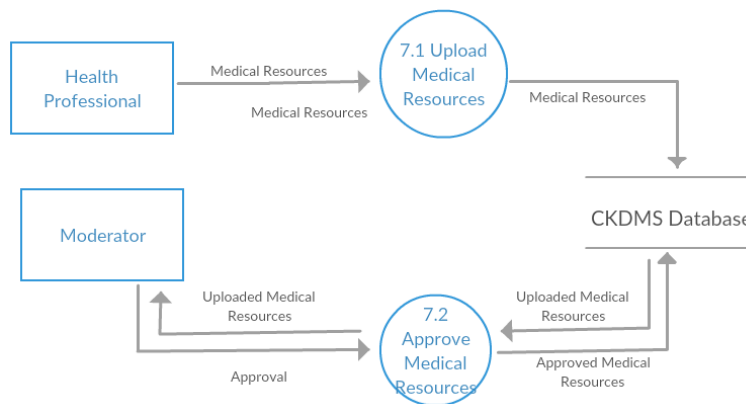
Figure 9: Sub-explosion for Manage Medical Resources Function of CKDMS
