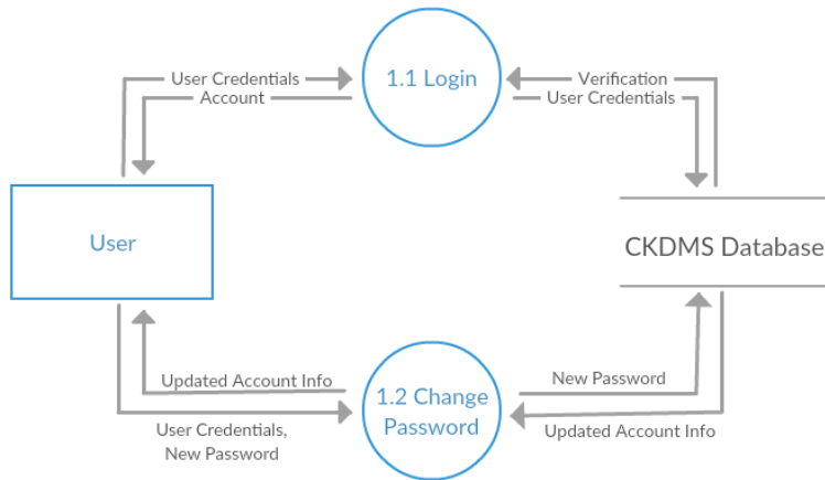
Figure 4: Sub-explosion for Login Function of CKDMS
