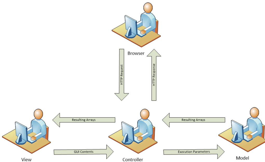
Figure 8: System Architecture
