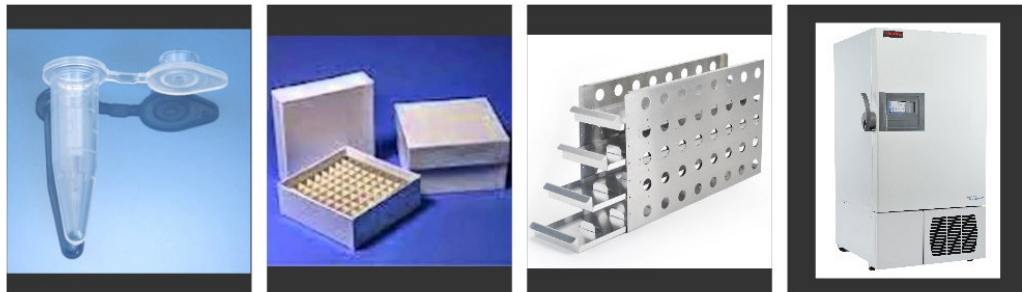
Figure 1: Freezer-Rack-Box Hierarchy
