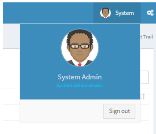
Figure 53: Sign Out
