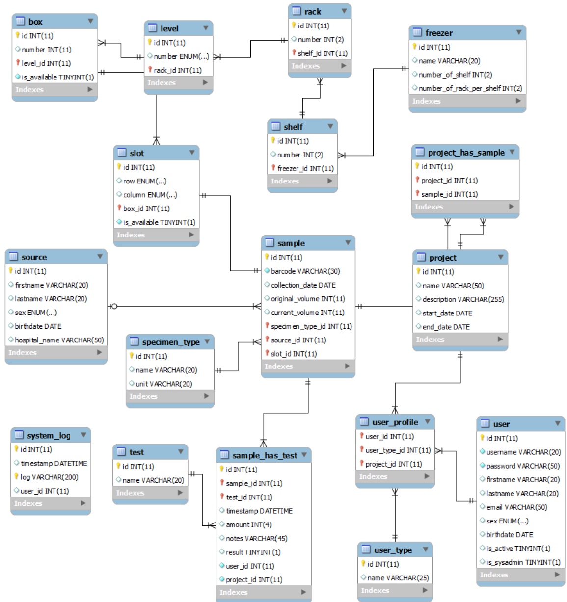
Figure 7: Entity-Relationship Diagram
