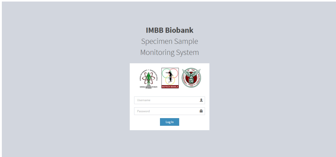
Figure 9: Login Page
