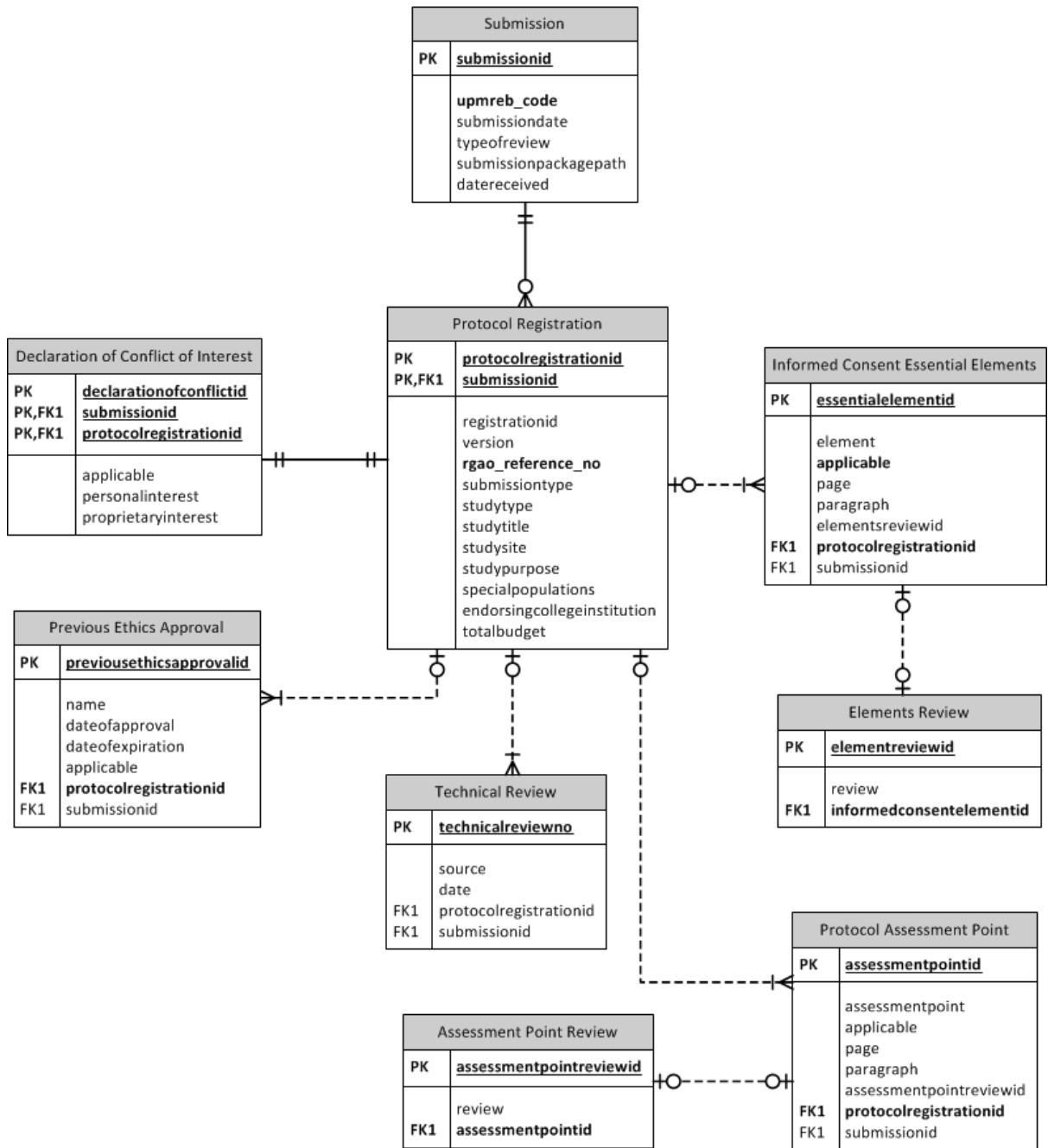
Figure 13.2. Entity Relationship Diagram
