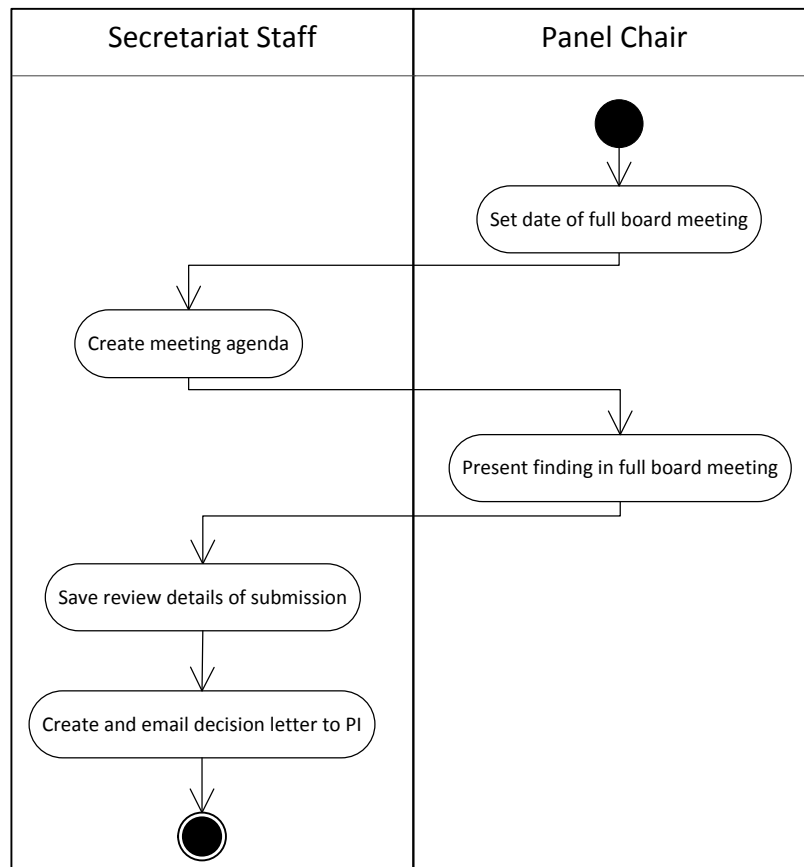
Figure 7. Activity diagram of full board meeting
