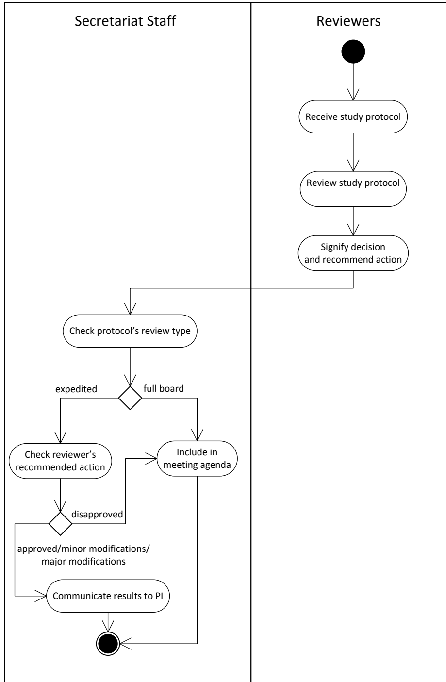
Figure 6. Activity Diagram of study protocol initial review
