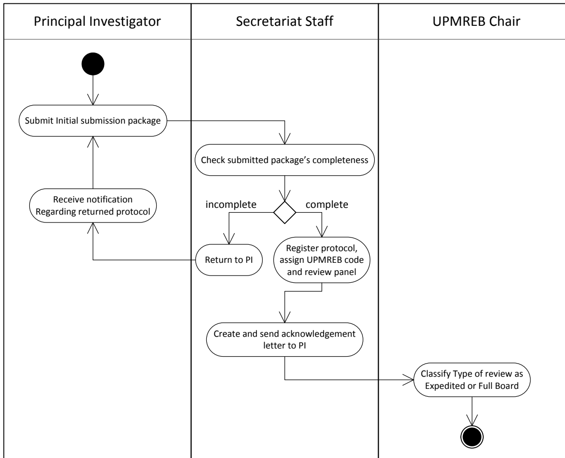
Figure 4. Activity diagram of initial submission
