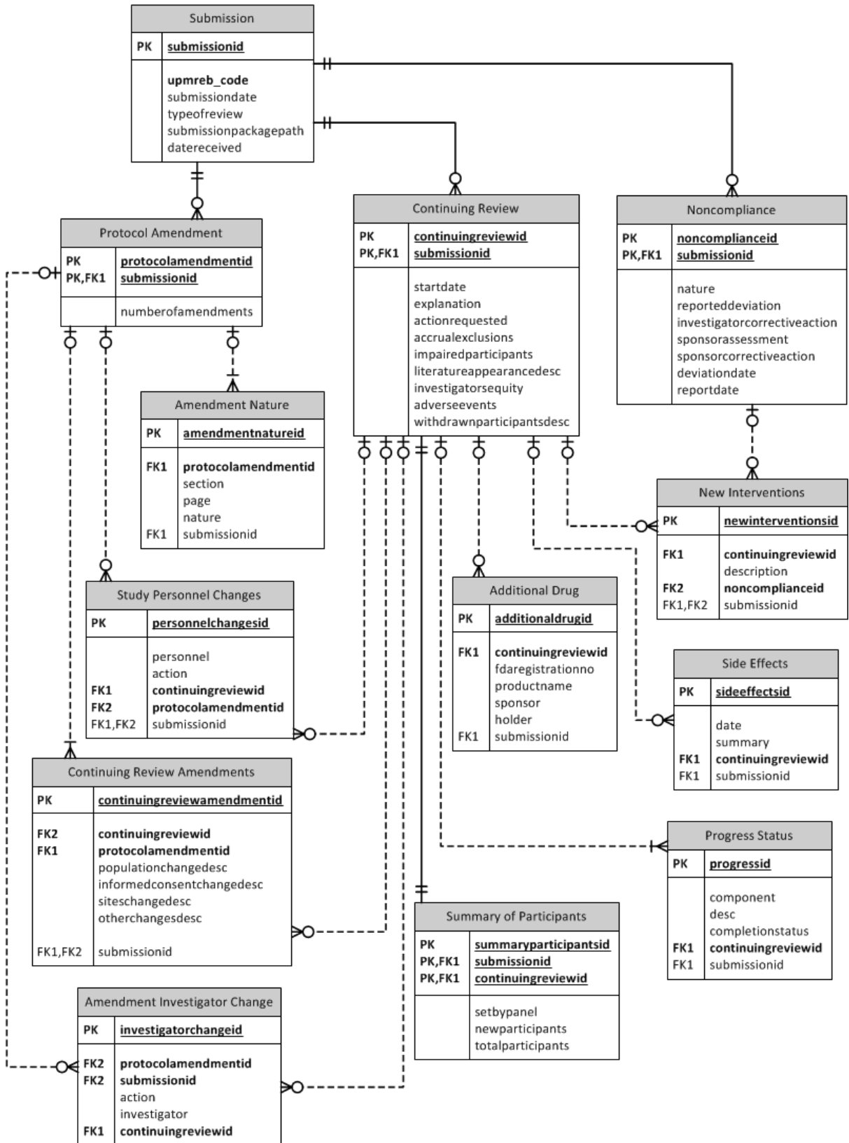
Figure 13.3. Entity Relationship Diagram
