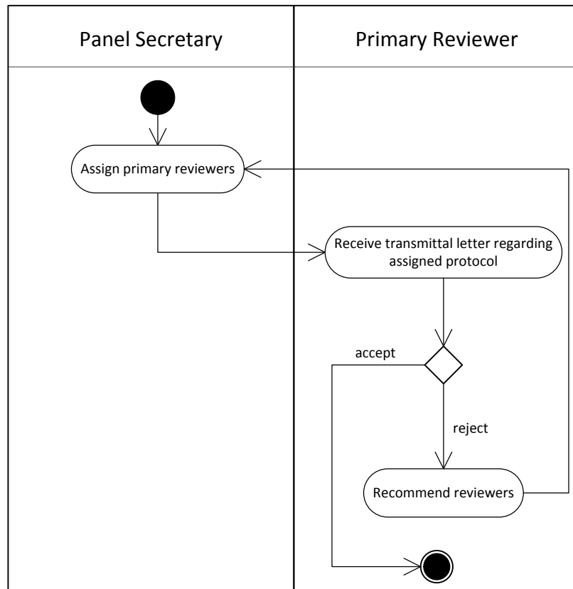
Figure 5. Activity diagram of assignment of reviewers
