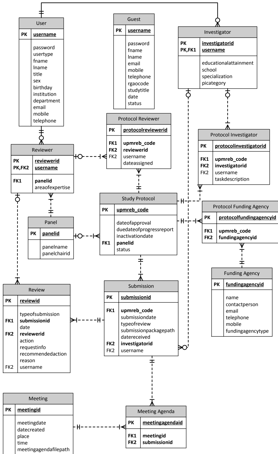
Figure 13.1. Entity Relationship Diagram
