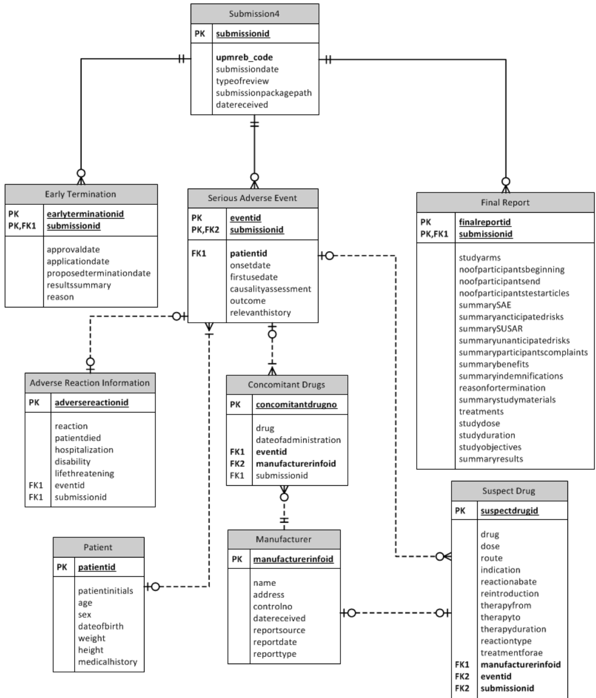
Figure 13.4. Entity Relationship Diagram
