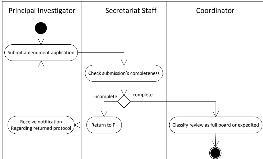
Figure 8. Activity diagram of submission of study protocol amendment application
