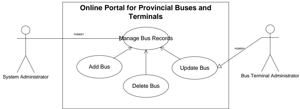
Figure 6. Manage Bus Records Use Case Diagram of the Online Portal for Provincial Buses and Terminals
