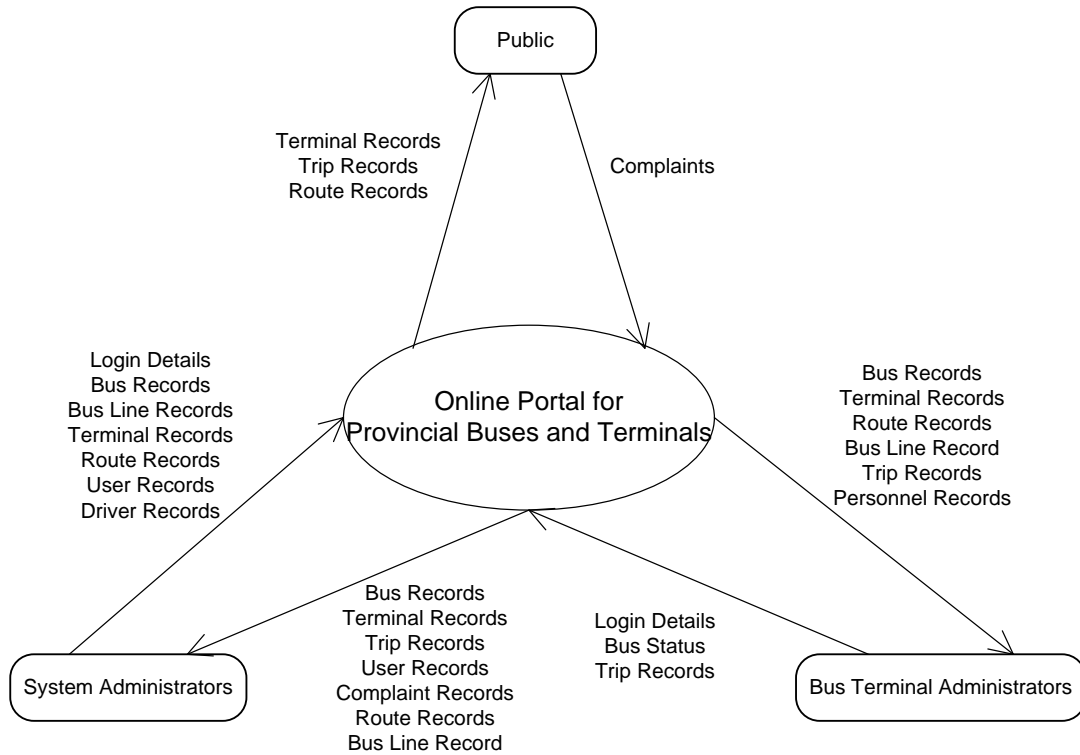
Figure 2. Context Diagram of the Online Portal for Provincial Buses and Terminals
