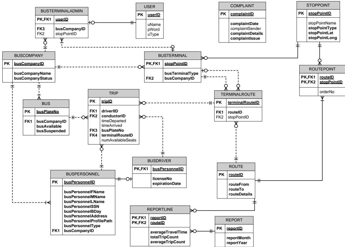
Figure 11. Entity Relationship Diagram of the Online Portal for Provincial Buses and Terminals
