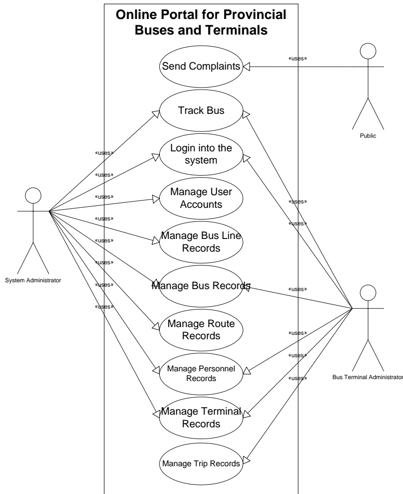
Figure 3. Top Level Use Case Diagram of the Online Portal for Provincial Buses and Terminals
