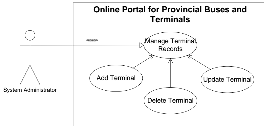
Figure 9. Manage Terminal Records Use Case Diagram of the Online Portal for Provincial Buses and Terminals
