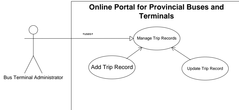
Figure 10. Manage Trip Records Use Case Diagram of the Online Portal for Provincial Buses and Terminals
