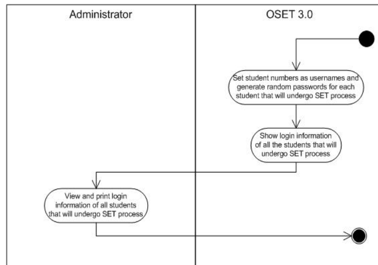
Figure 25: Activity Diagram(Automatic creation of user account for students)
