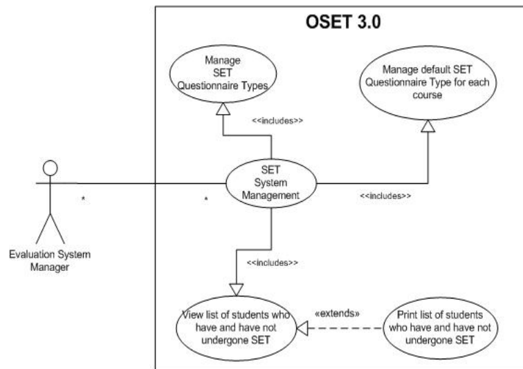
Figure 12: Use Case(SET System Management)
