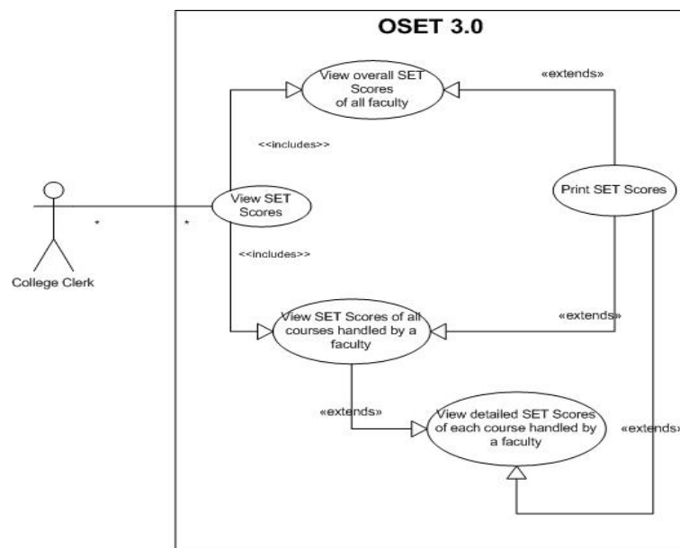
Figure 10: Use Case(View SET Scores)
