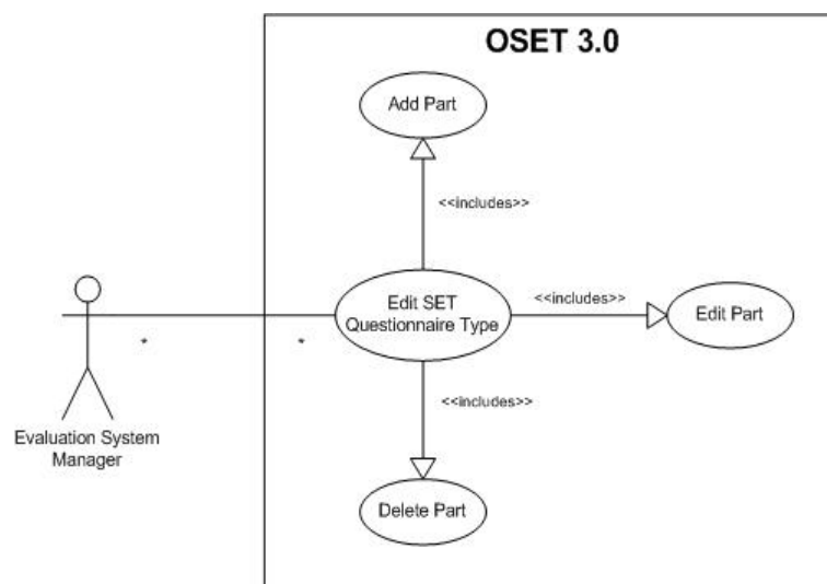
Figure 14: Use Case(Edit SET Questionnaire Type)
