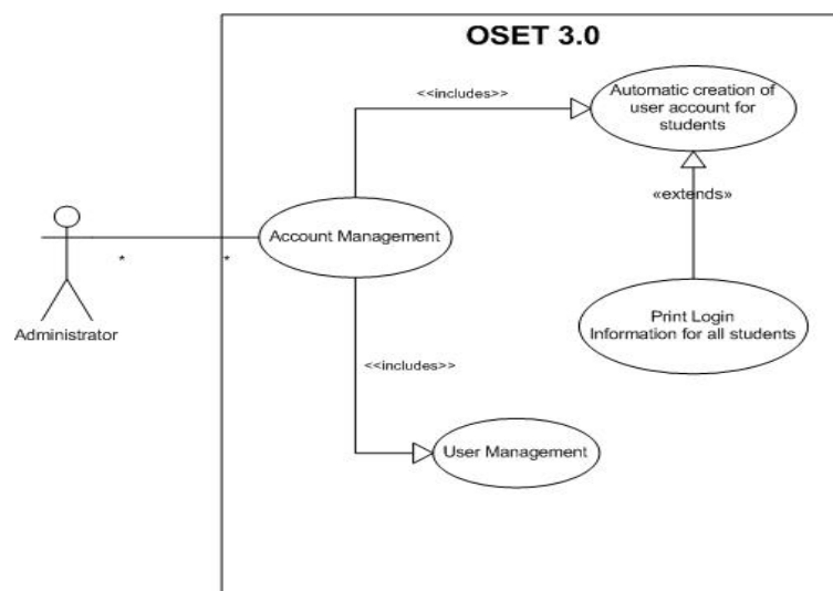
Figure 24: Use Case(Account Management)
