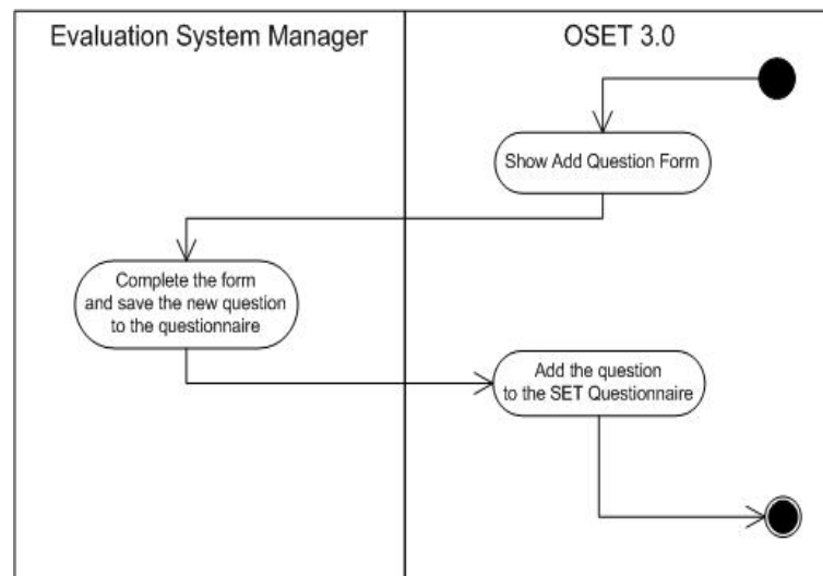
Figure 19: Activity Diagram(Add question to a SET Questionnaire Part)
