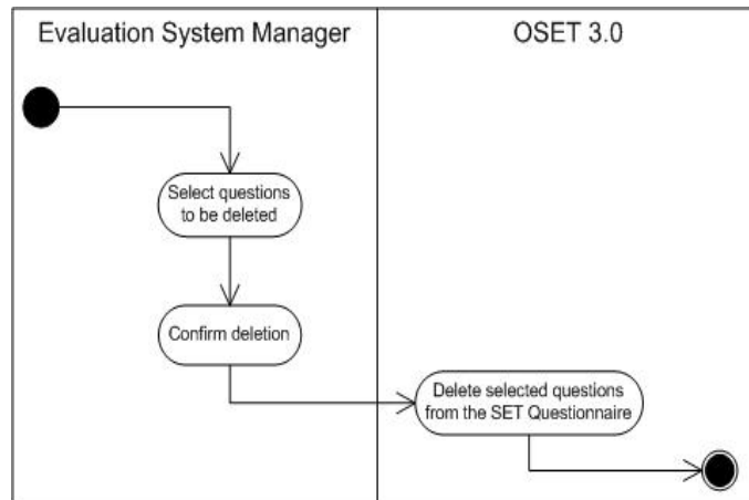
Figure 18: Activity Diagram(Delete question From a SET questionnaire Part)
