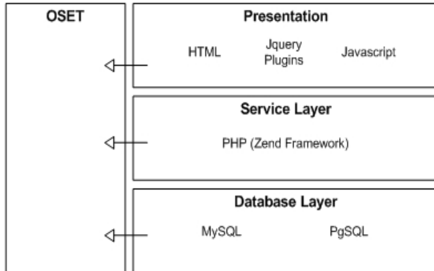
Figure 31: OSET 3.0 System Architecture
