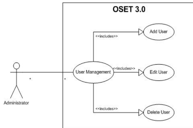
Figure 26: Use Case(User Management)
