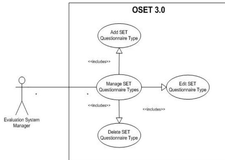
Figure 13: Use Case(Manage SET Questionnaire Types)
