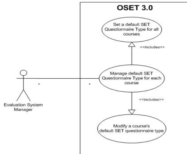
Figure 21: Use Case(Manage default SET Questionnaire Type for each course)
