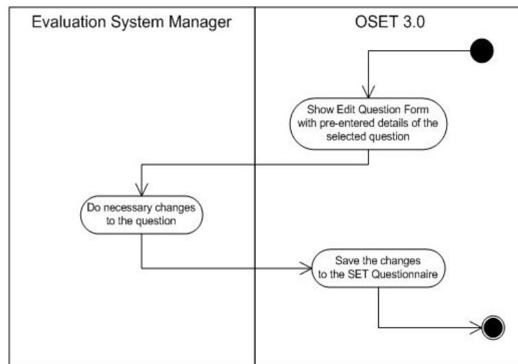
Figure 20: Activity Diagram(Edit question from a SET Questionnaire Part)
