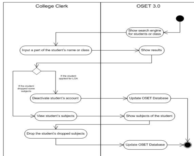
Figure 11: Activity Diagram (Management of students who will evaluate)
