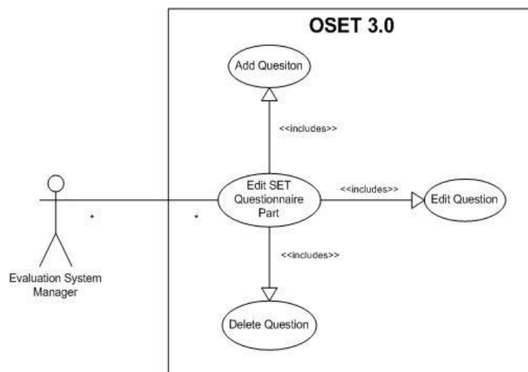
Figure 17: Use Case(Edit SET Questionnaire Parts)
