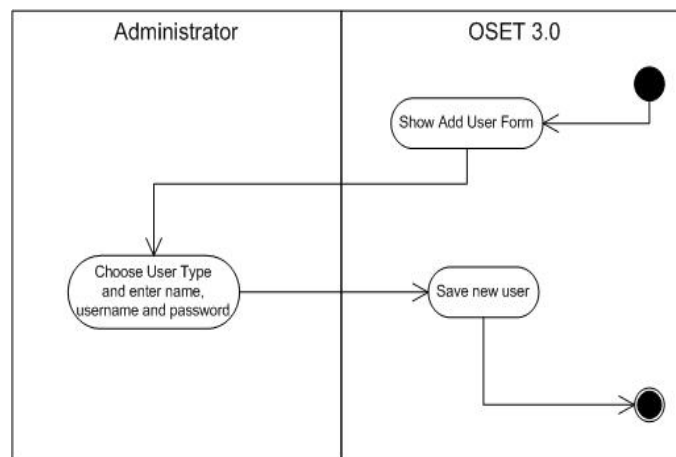
Figure 27: Activity Diagram(Add user)
