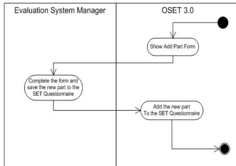
Figure 16: Activity Diagram(Add Part to a SET Questionnaire)
