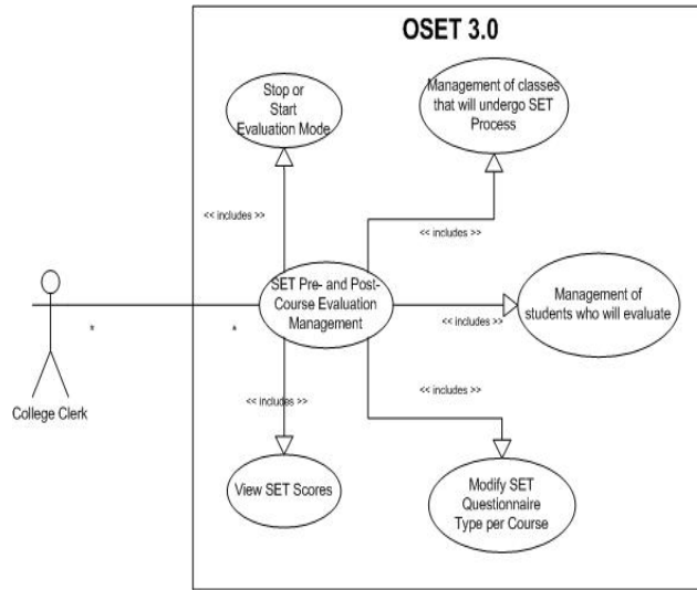
Figure 5: Use Case(SET Pre- and Post- Course Evaluation Management)
