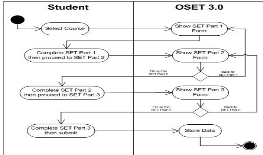
Figure 4: Activity Diagram: Course Evaluation
