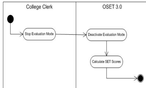
Figure 7: Activity Diagram(Stop Evaluation Mode)
