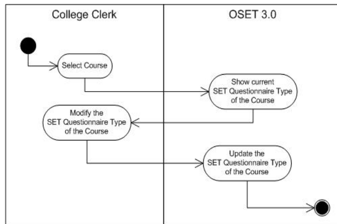
Figure 9: Activity Diagram(Modify SET Questionnaire Type per Course)
