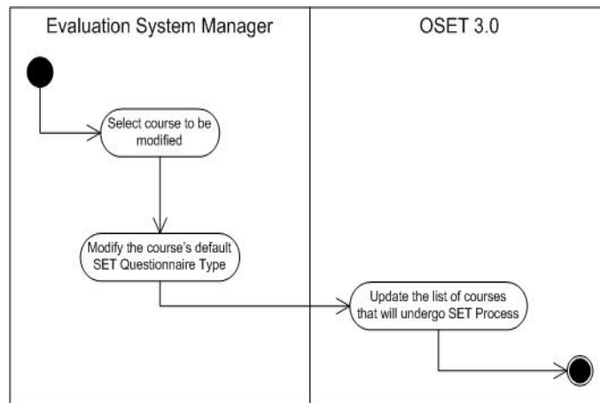
Figure 23: Activity Diagram(Modify a course's default SET Questionnaire Type)
