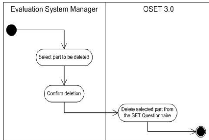
Figure 15: Activity Diagram(Delete Part from a SET Questionnaire)
