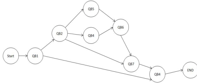
Figure 2: Deterministic Finite Automaton of SurveyProject 2001
