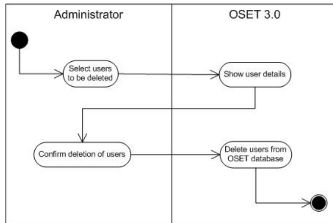
Figure 28: Activity Diagram(Delete users)
